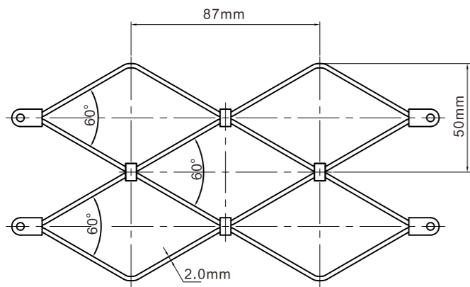
The material:304/316 The wire diameter:2.0mm Mesh size:50*87mm Mesh sheet form:KL24
