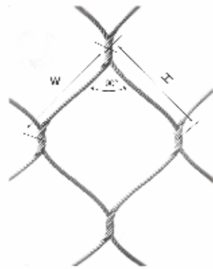
The material:304/316 The wire diameter:2.0mm Mesh width(W=H):60mm
